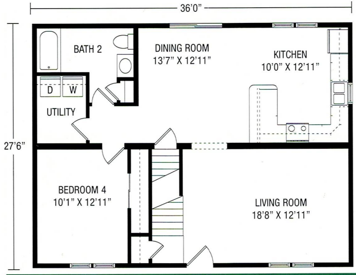
Plan No. 633 ♦ 1690 SQ. FT.
